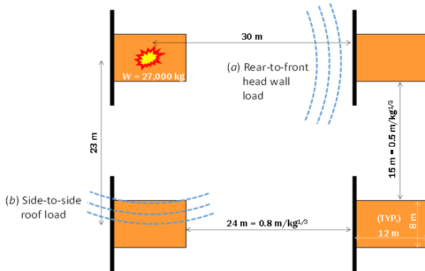
Figure 4: Dimensions and layout of ECMs for sample calculation.
