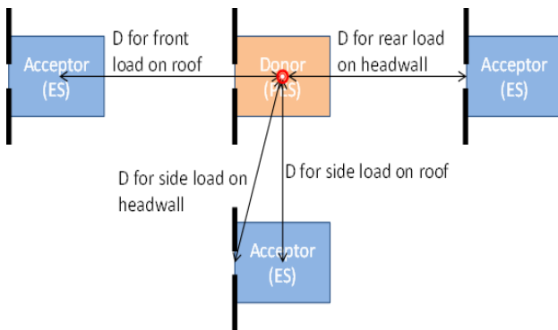
Figure 2: Examples of definition of distances for blast load computations.
