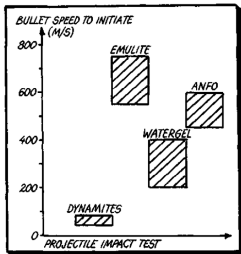
Figure 1 Bullet impact tests on a range of explosives
