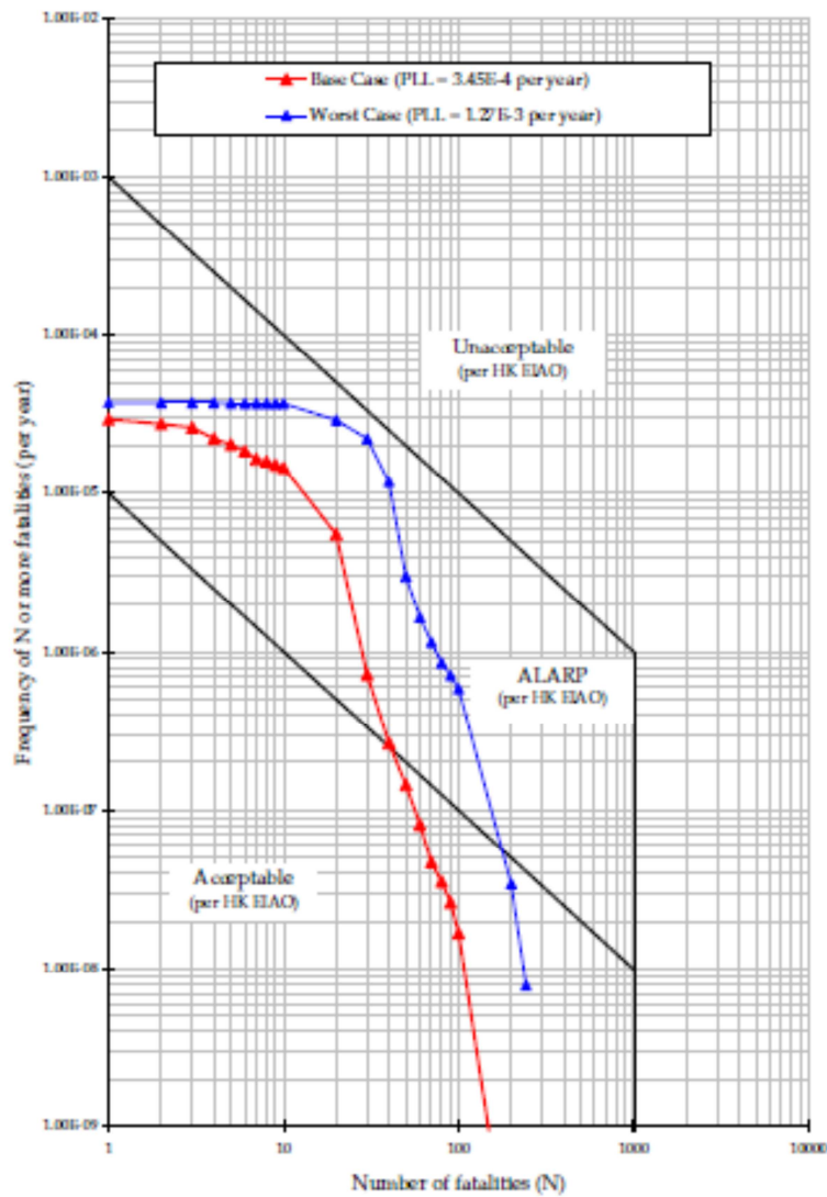
Figure 4 Overall Fatality Frequency vs number of fatalities for the transport of emulsion explosives for a base case and a worst case incorporating a 20% increase in the number of deliveries of explosives.
