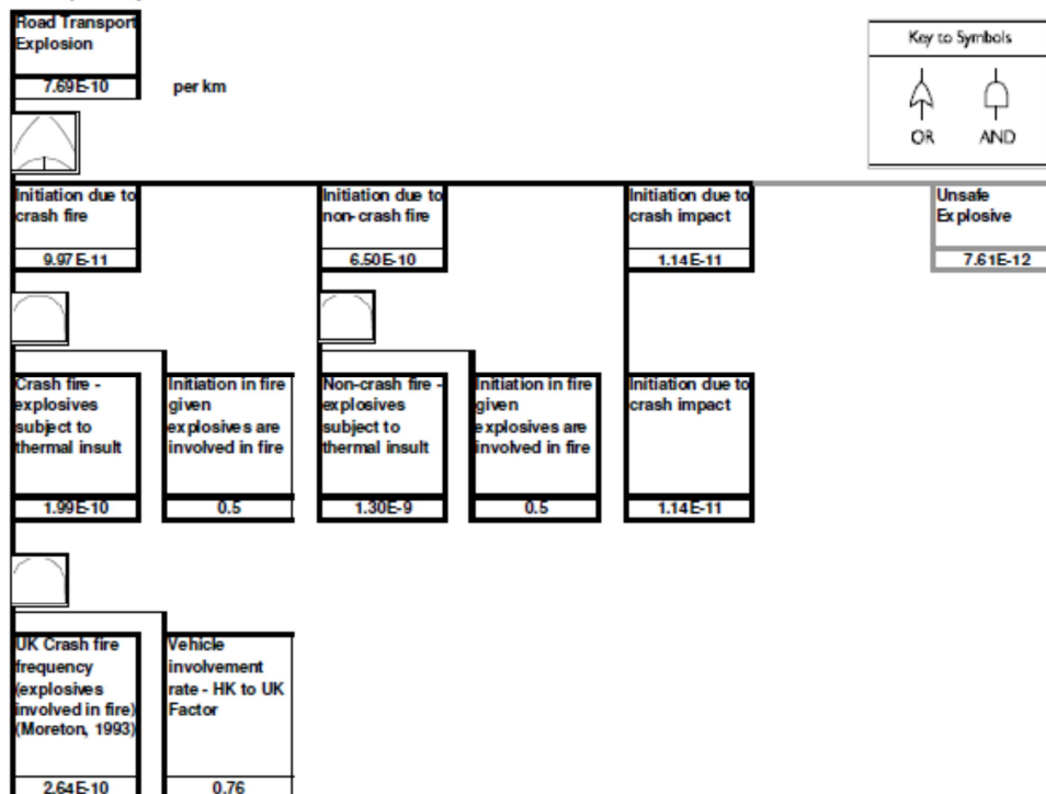
Figure 2 Fault trees – Truck Explosion Frequency per truck per km – Expressway and non-Expressway travel normalised to match UK and Hong Kong crash frequencies.
