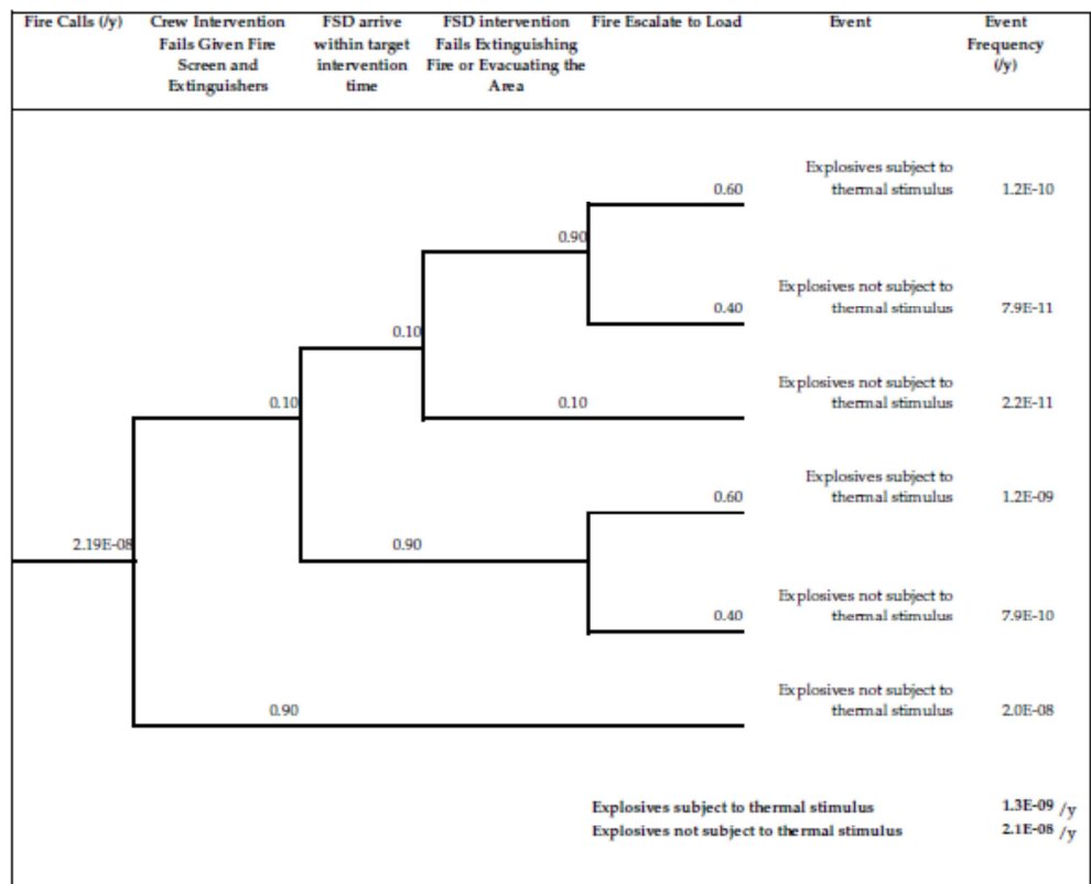
Figure 3 Event Tree for non crash fire scenario
